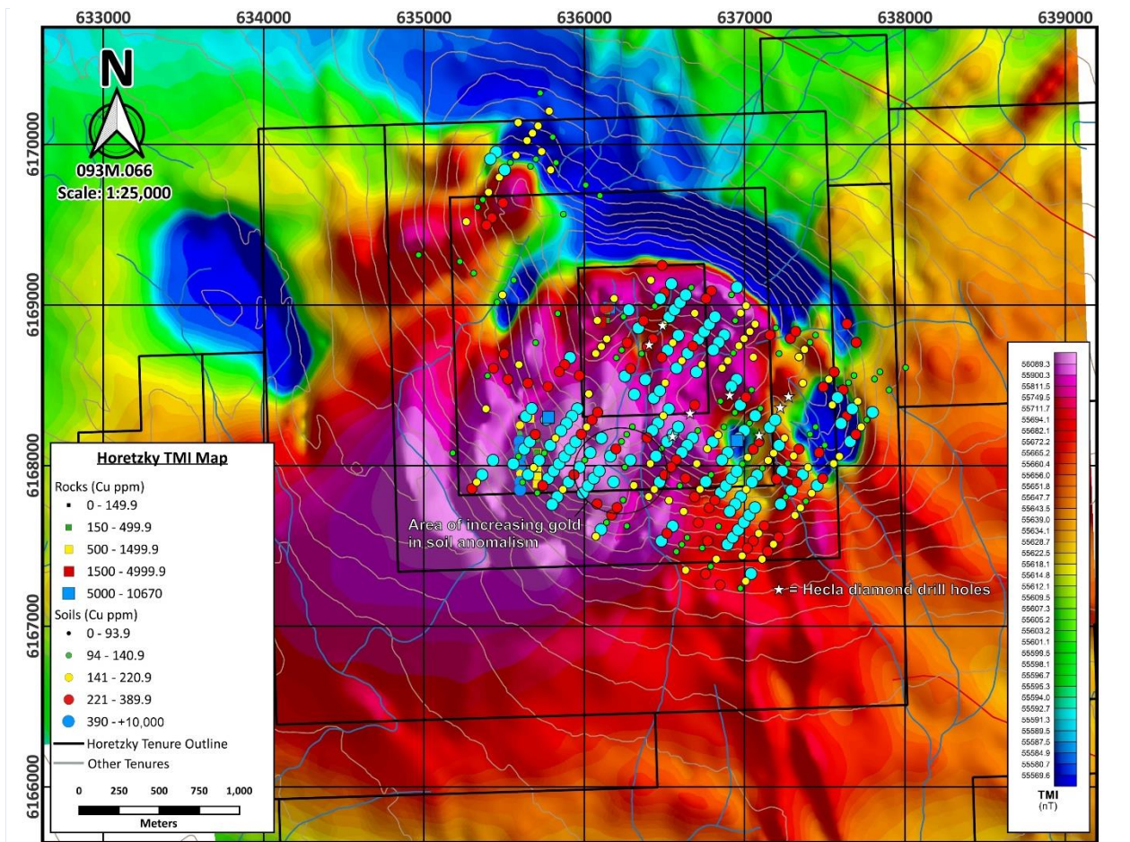
Figure 2 – Surface geochemistry on total magnetic intensity airborne magnetics.
