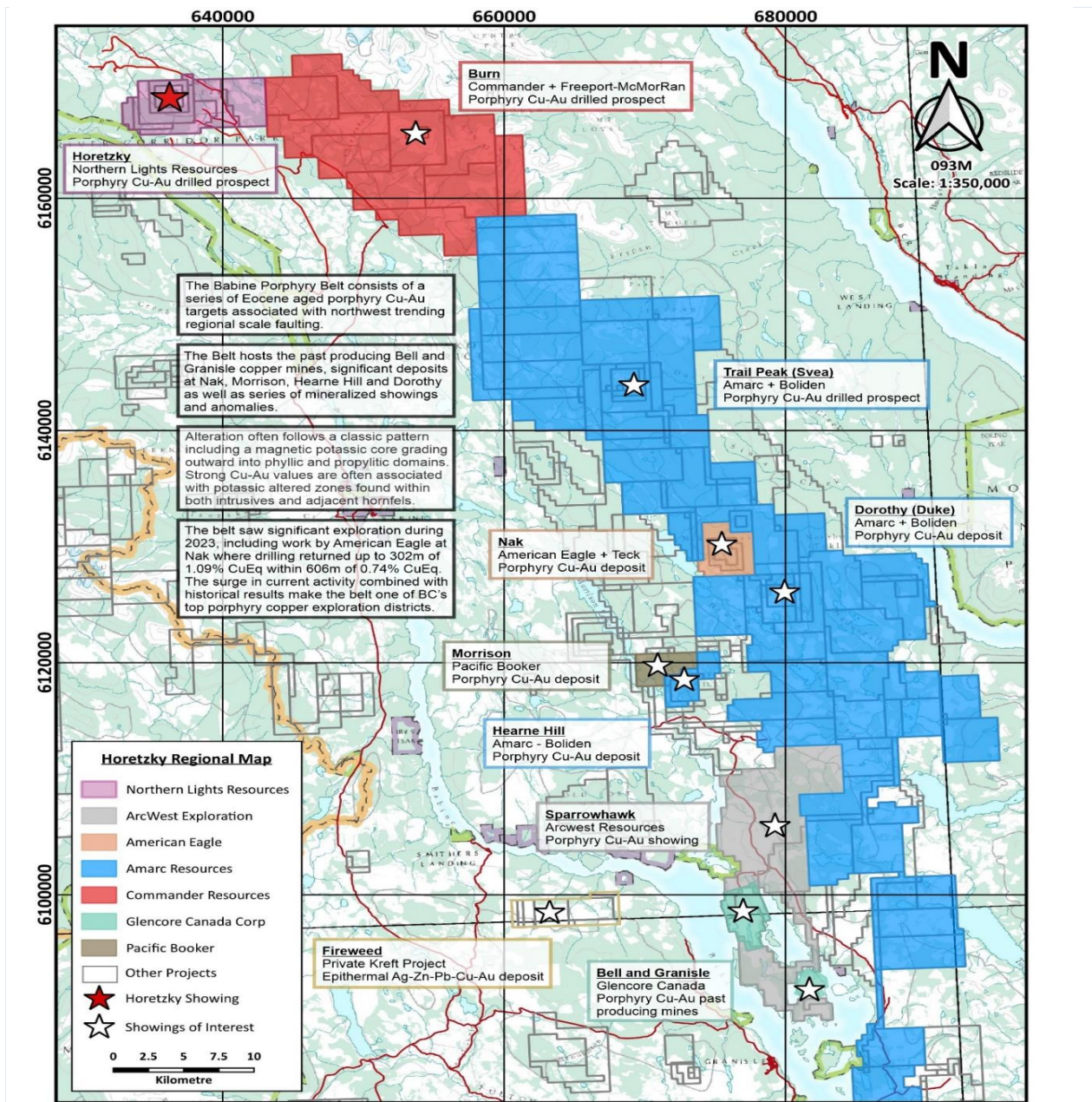
Figure 1 – Location of the Horetzky Project within the Babin Porphyry Belt
